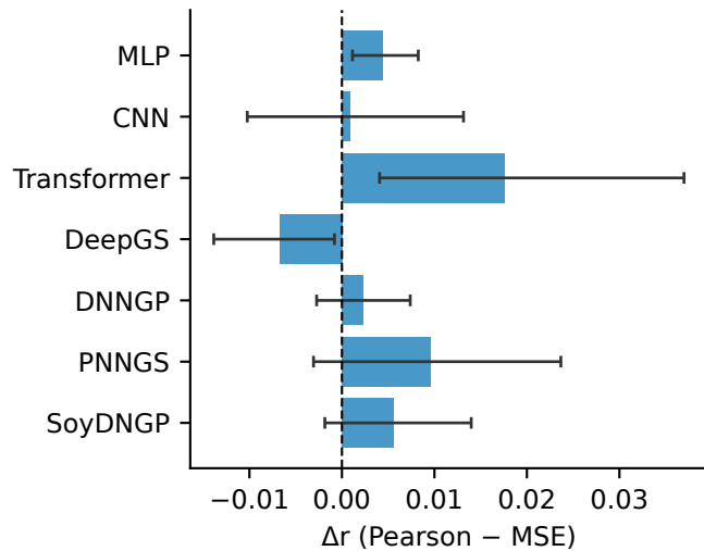
Main ablation: 7 networks
