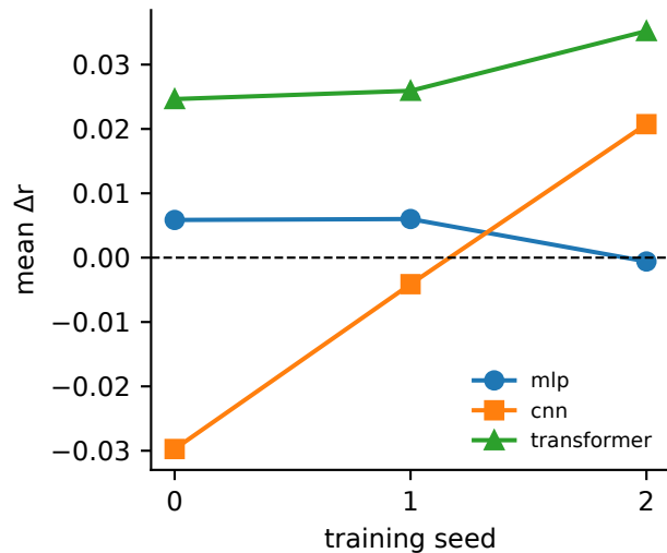
Initialization sensitivity
