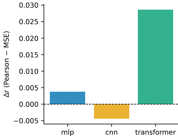
Nested HPO: 3-network subset
